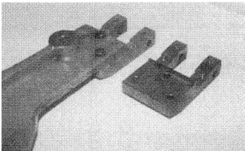
Updated drum finger spider and replaceable finger.
